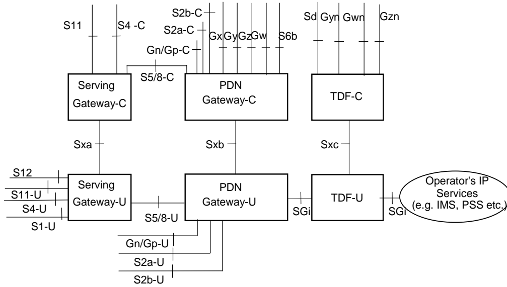
Figure 29. Architecture reference model with CUPS.
