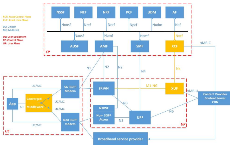
Figure 18. 5G System Architecture alternative 2.
