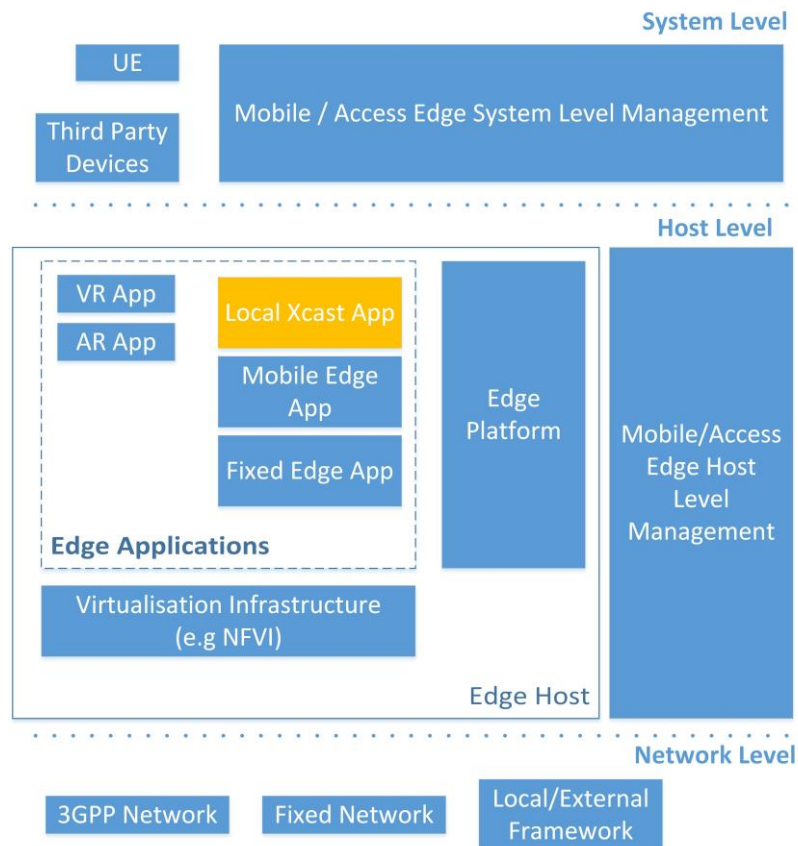
Figure 14: Mobile edge computing framework adapted to multi-access.
