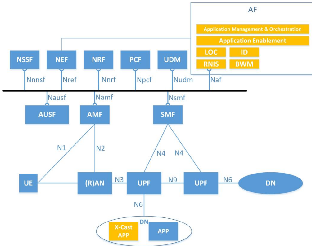
Figure 16: MEC in 5G system architecture.
