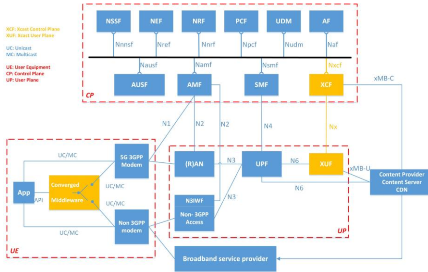
Figure 17. 5G System Architecture alternative 1.
