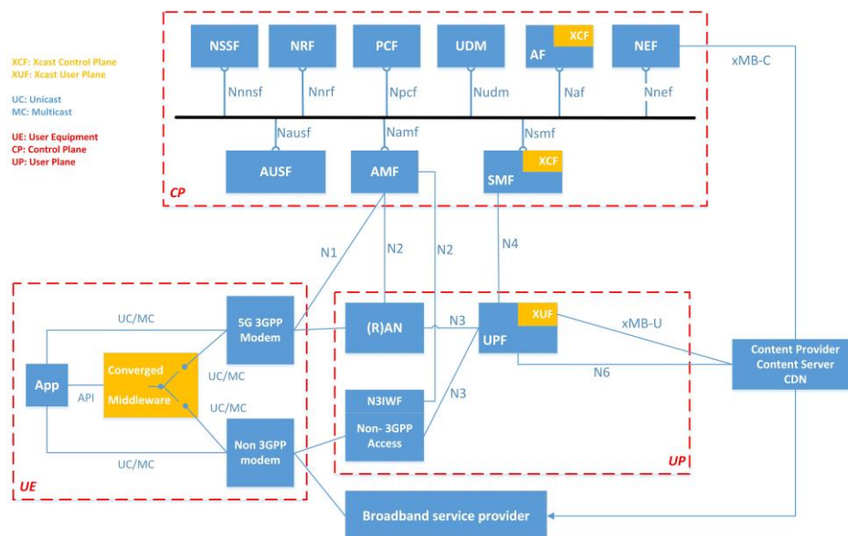
Figure 21. 5G System Architecture alternative 3.
