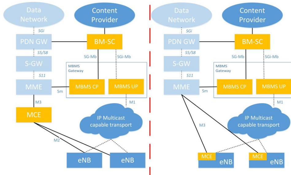
Figure 2: Centralized versus Distributed MCE deployment.
