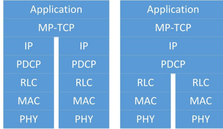
Figure 11. Options for integrating multi-connectivity into 5G networks.
