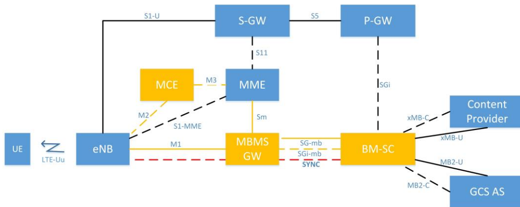
Figure 1: eMBMS Architecture.
