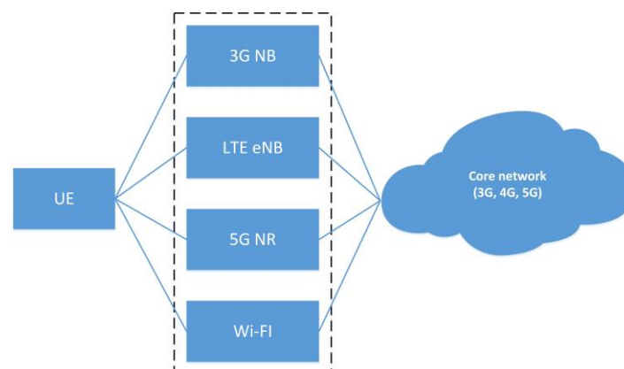
Figure 10. 5G architecture with Multi-connectivity.
