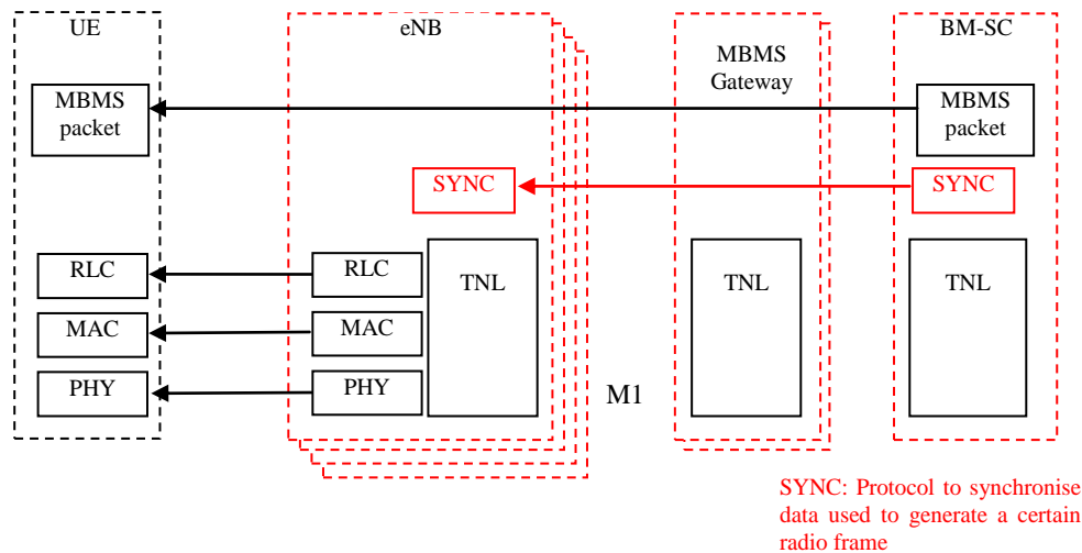
Figure 26: Overall u-plane architecture of the MBMS content synchronization.
