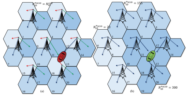
Fig. 4. Cell scrambling sequence initialization N_{ID}^{n_{SCID}} according to the physical layer cell ID (a), and given by the higher-layer parameter DL-DMRS-Scrambling-ID (b).
